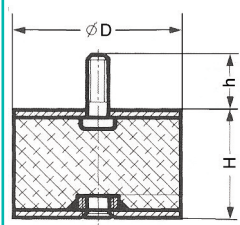
Abb. 1 Druckelement (Puffer) Compression element
