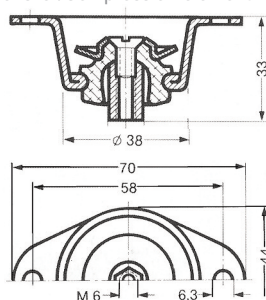
Abb.3 Glockenelement. / Bell element
